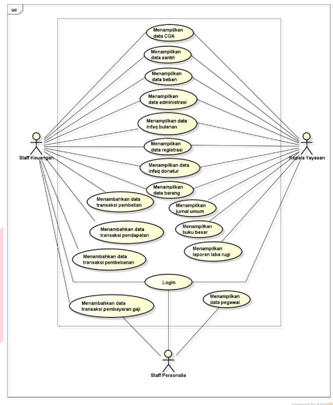
GAMBAR 1-3 UseCase Diagram
