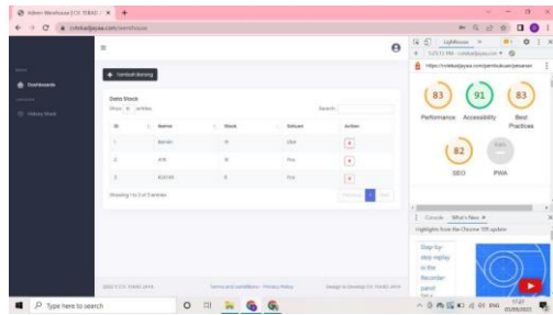
Gambar 4. 17 Pengujian LightHouse Admin Gudang
