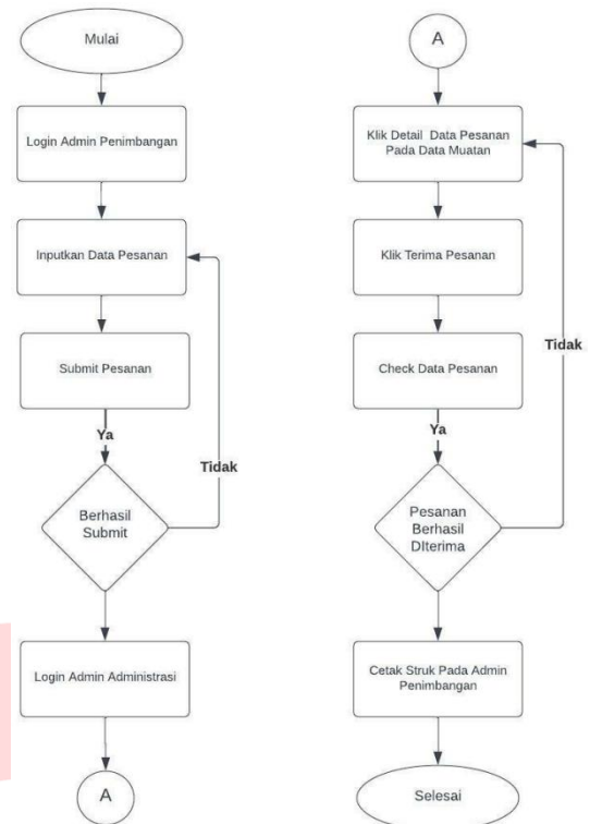
Gambar 3. 10 Alur Pengiriman Data
