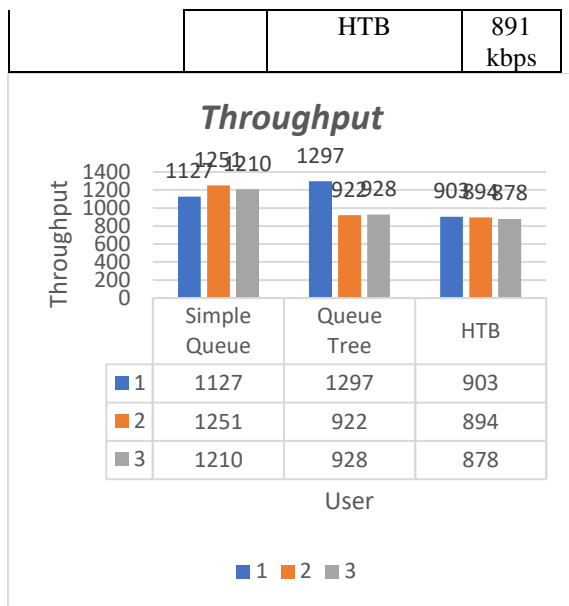
Gambar 12. Grafik Throughput
