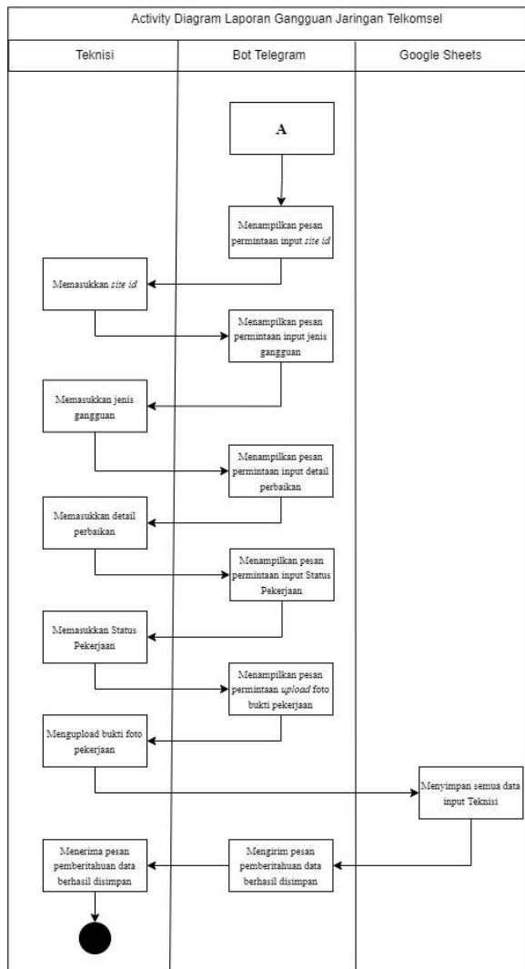
Gambar 4 Activity Diagram
