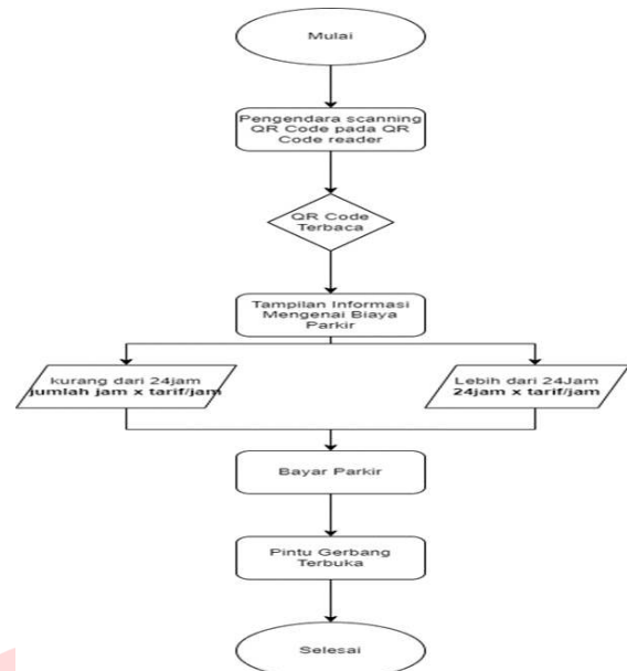
Gambar 3.4 Flowchart Payment
