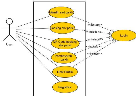
Gambar 3. 5 Use Case
