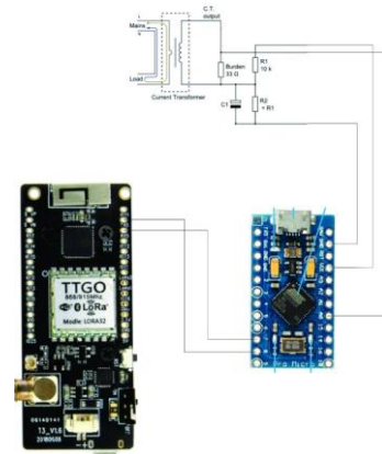
Gambar 3. 4 Schematic perancangan alat transmitter
