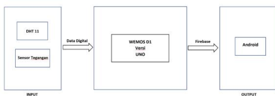
Gambar 3. 4 Diagram Blok Sistem Monitoring Baterai OpzV
