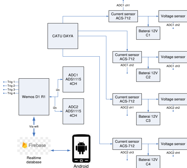
Gambar 3. 3 Model Sistem Monitoring Baterai OpzV
