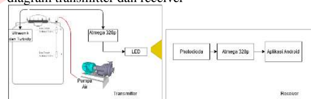
Gambar 8 Blok Sistem Transmitter dan Receiver
