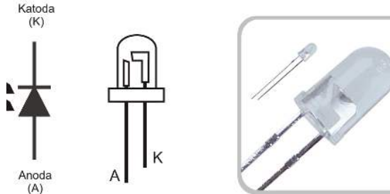
Gambar 6 Photodiode
