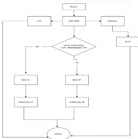
Gambar 3. 1 Flowchart Sistem
