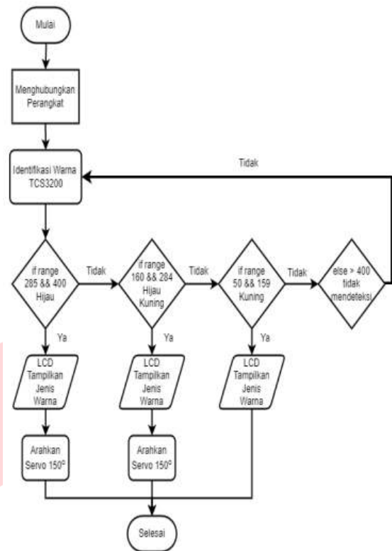
GAMBAR 2. 2 flowchart
