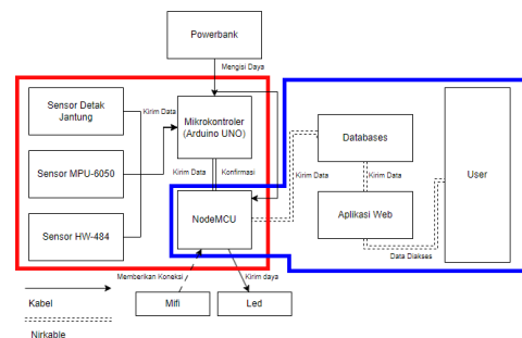
GAMBAR 1 Blok Diagram
