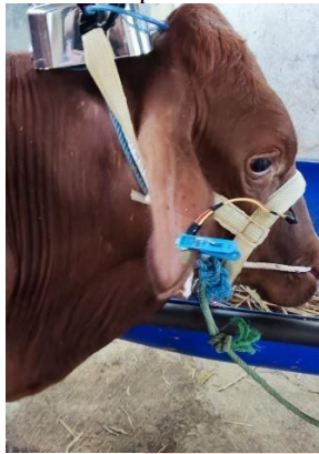
GAMBAR 7 Purwarupa Alat
