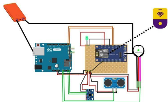
GAMBAR 1 Perancangan Hardware
