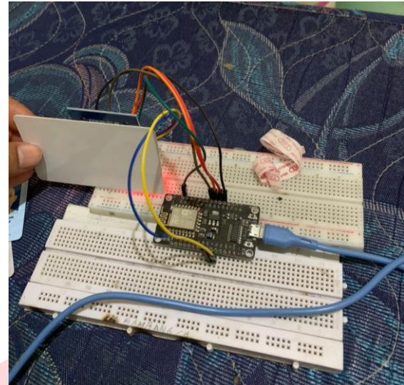
Gambar 8 Scanning RFID
