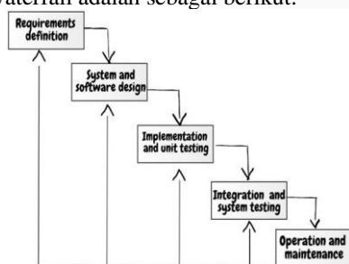
GAMBAR 1 Metode Waterfall
