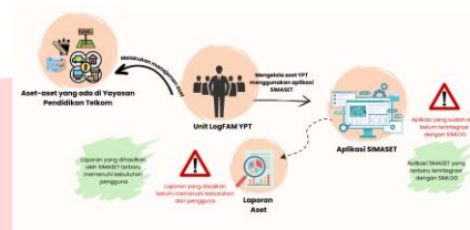
GAMBAR 2 Rich Picture
