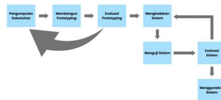
GAMBAR 1 Metode Prototype
