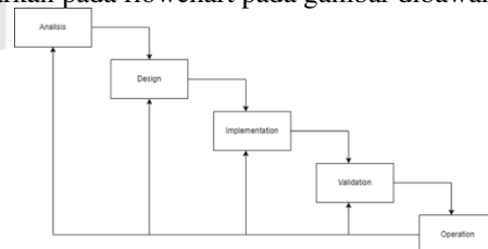
GAMBAR 3.1 Metode Waterfall
