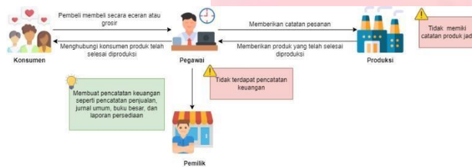
GAMBAR 3 – 1 Rich Picture
