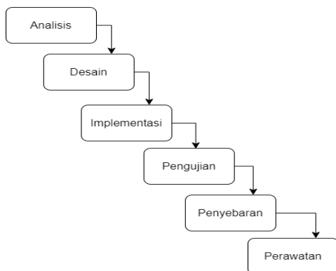
Gambar 2 - 1 Waterfall Diagram
