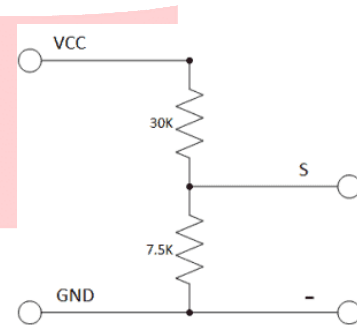
Gambar 1. 3 Sensor Tegangan
