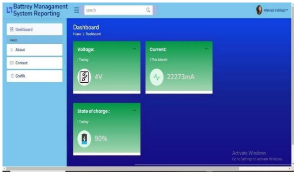
Gambar 3. 1 Purwarupa website
