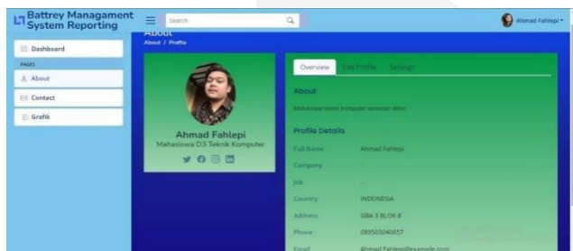
Gambar 3. 3 Halaman About
