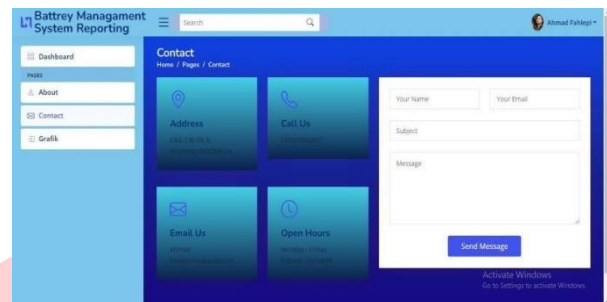
Gambar 3. 5 Halaman Contact
