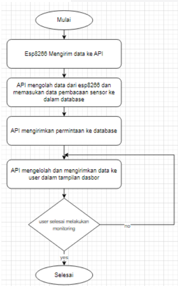
Gambar 2. 2 flowchart
