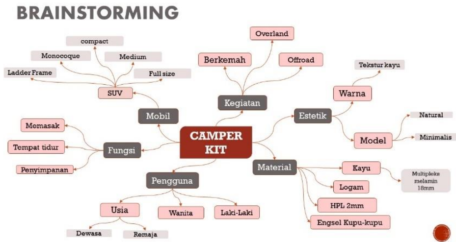
Gambar 1 Mind Mapping
