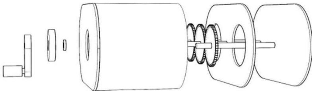
Gambar 6 Exploded View
