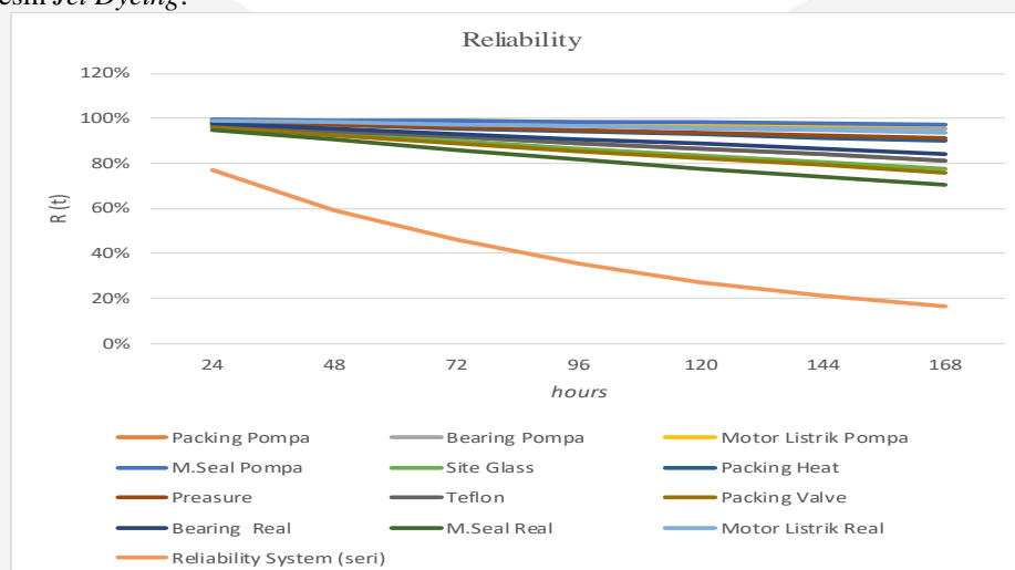
Gambar 6 Grafik hasil perhitungan Analytical Approach Reliability
