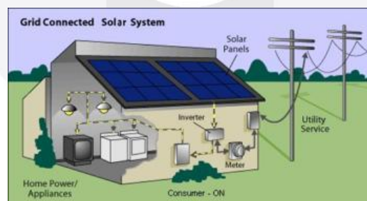
Gambar II- 3. Gambar Sistem On Grid
