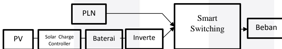
Gambar II-1. Smart Switching
