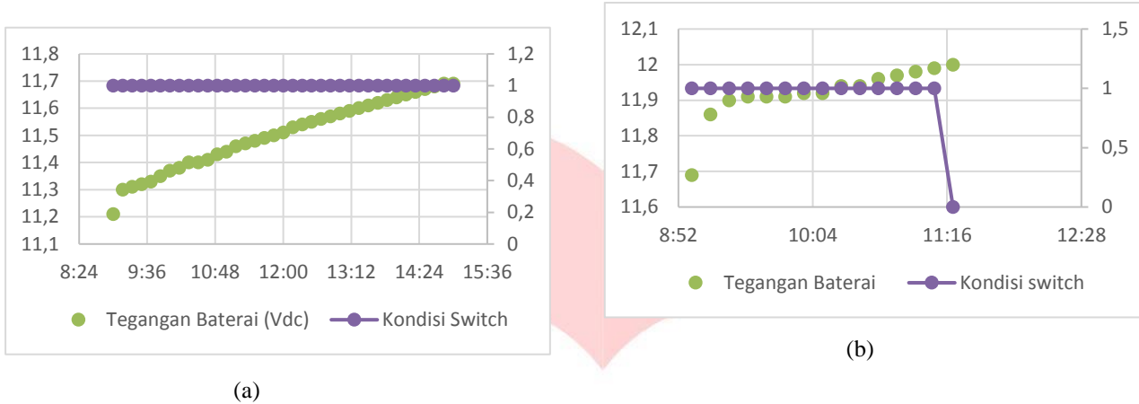
Gambar III- 2 Pengujian switching saat charging
