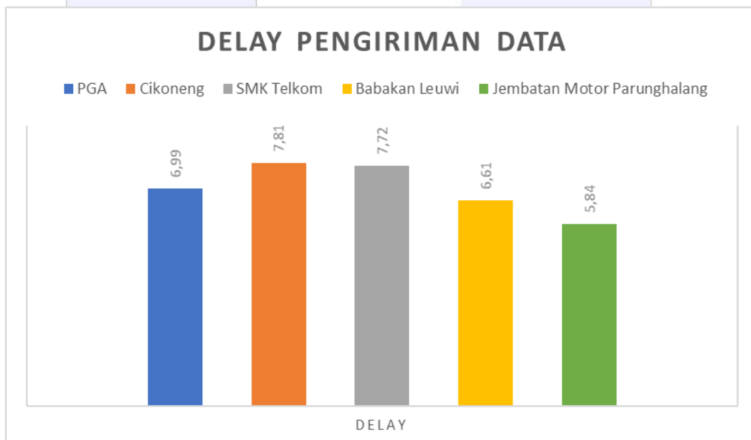
Gambar 4.1.2 Delay Pengiriman Data
