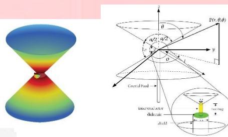
Gambar 2. Antena Biconical .
