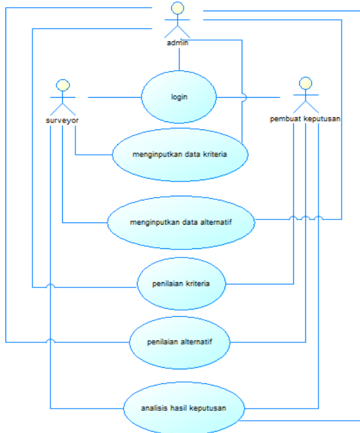
Gambar 4. Usecase diagram
