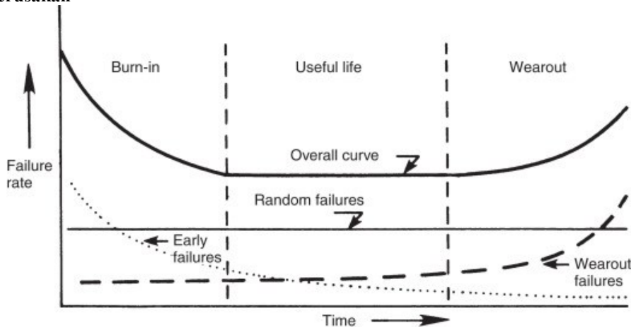
Gambar II.1 Bathub Curve
