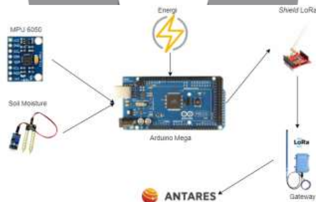
Gambar 2. Sensor Device
