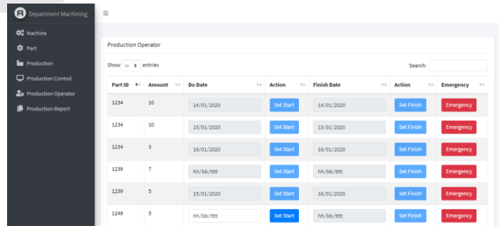
Figure IV.7 Operator Menu
