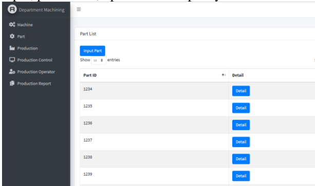
Figure IV.1 Input Menu
