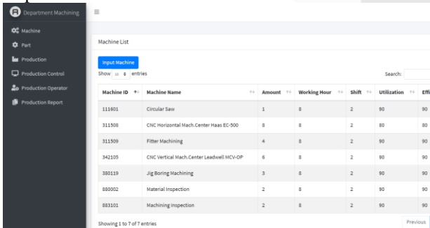
Figure IV.3 Machine List
