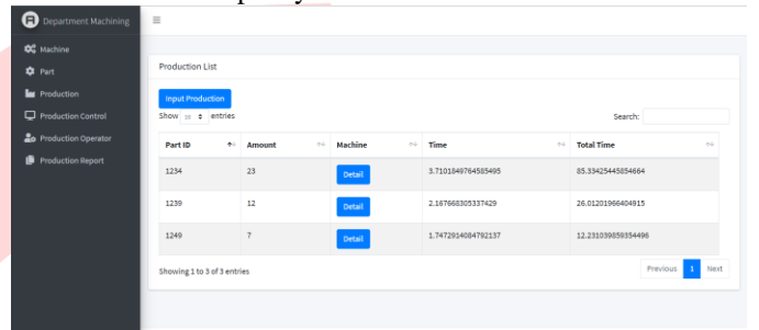
Figure IV.5 Production Menu
