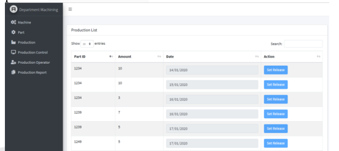
Figure IV.6 Production Control
