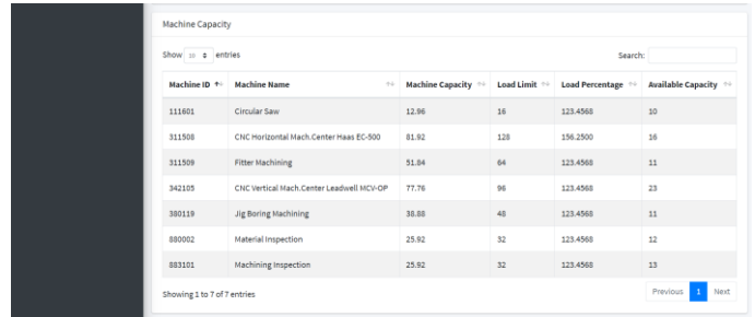
Figure IV.4 Capacity Calculation
