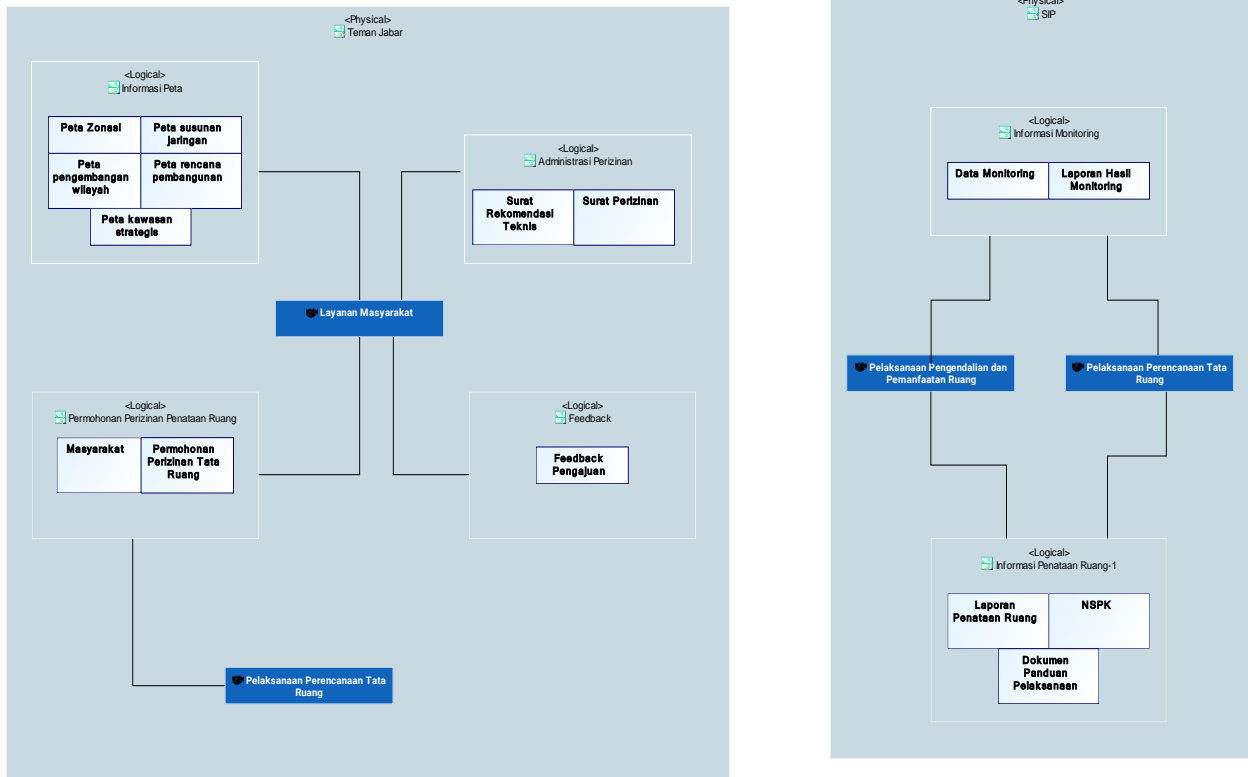
Gambar 5 Data Dissemination
