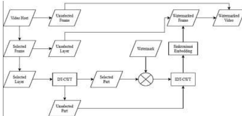
Gambar 2. Blok diagram proses embedding
