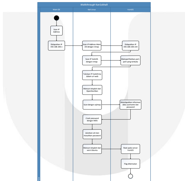
Gambar 4 Hasil Perumusan Activity Diagram Berdasarkan Walkthrough
