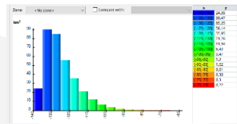
Gambar 4.4 Data hasil prediksi Signal Level
