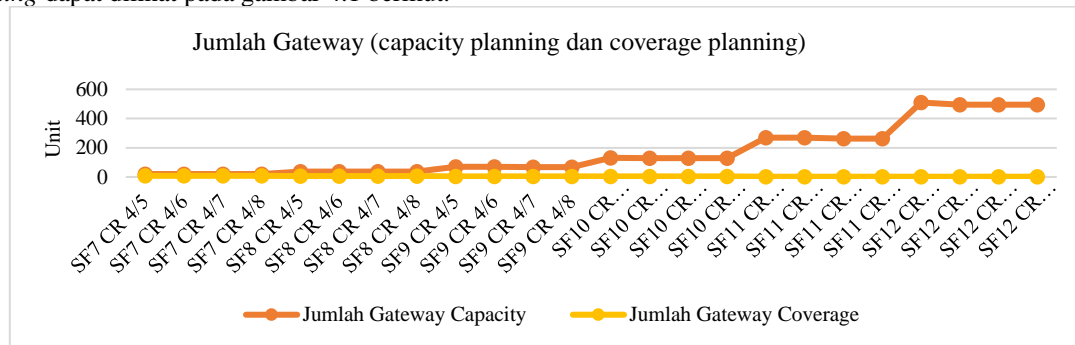
Gambar 4.1 Grafik jumlah gateway ( capacity planning dan coverage planning )
