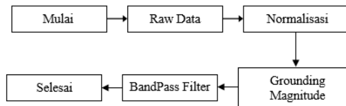
Gambar 3.2 Diagram blok pre-processing
