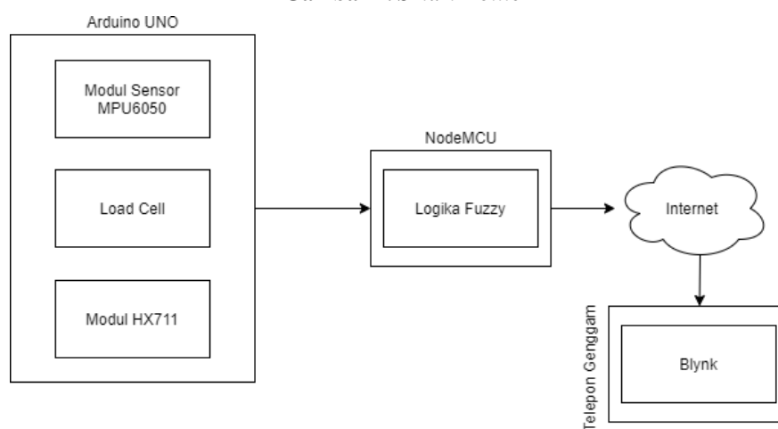
Gambar 2. Smart Bottle
