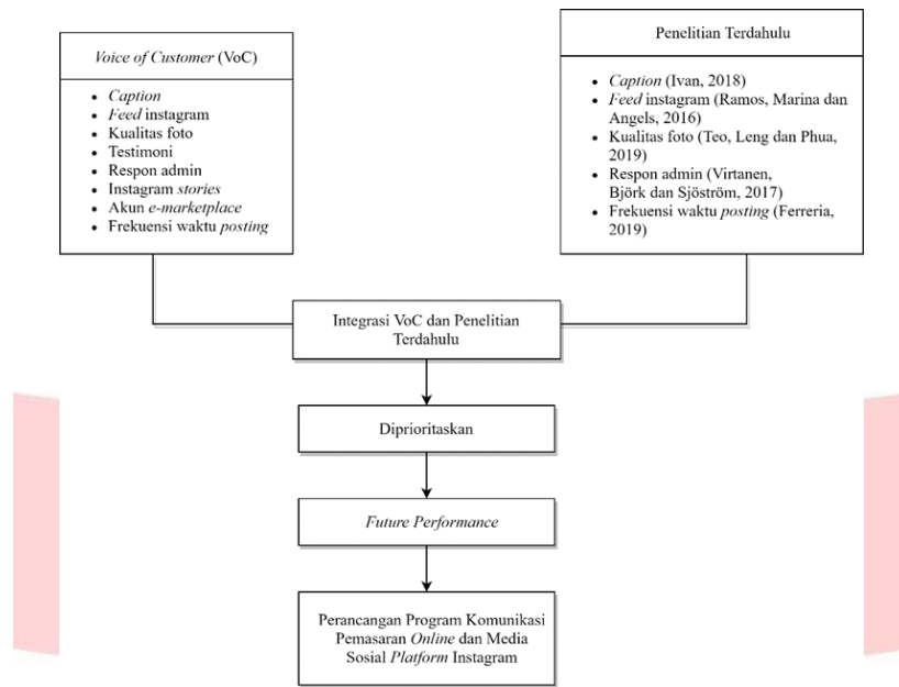
Gambar 2 Model Konseptual
