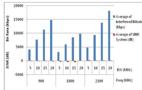
Figure 6.4 LTE interfered GSM1800
