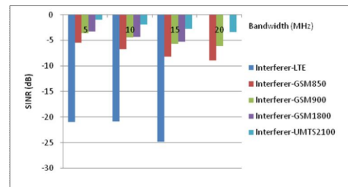
Figure 5.2 SINR for frequency 1800MHz
