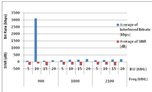
Figure 6.1 LTE interfered by LTE; Throughput vs SINR
