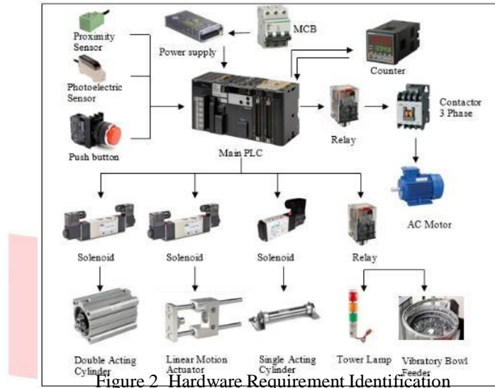
Figure 2 Hardware Requirement Identification
