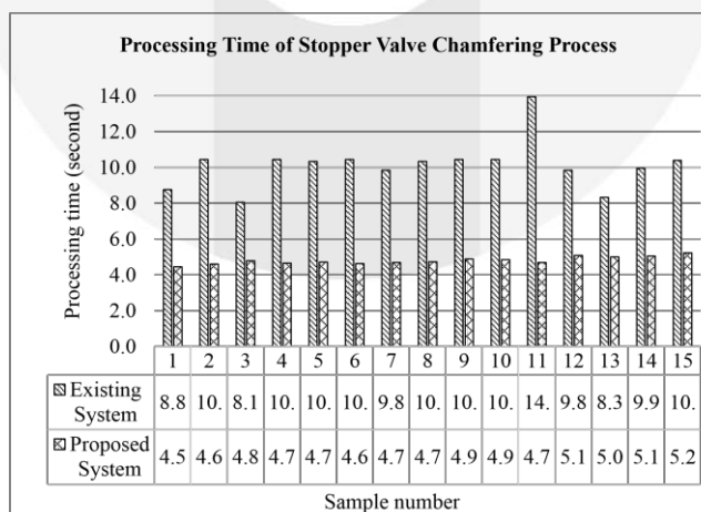
Figure 6 Processing Time of Stopper Valve Chamfering Process
