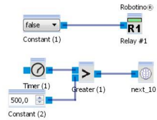
Figure IV.6 Gripper Off
