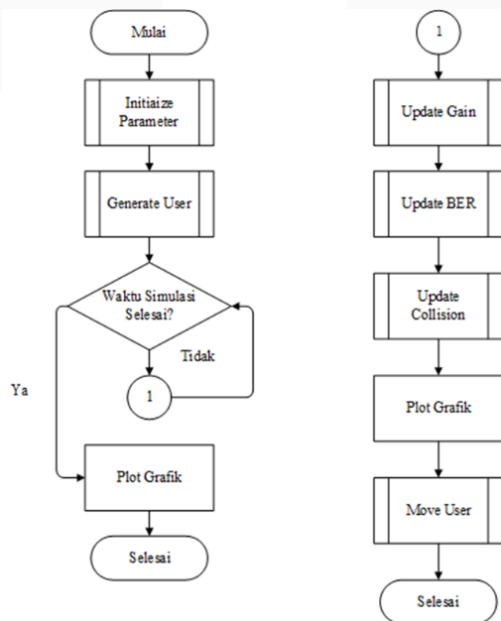
Gambar 4. Alur Simulasi System-Level.
