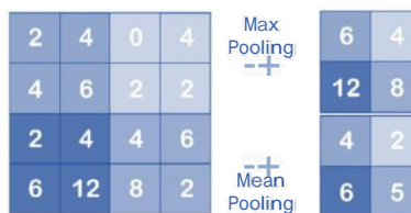
Gambar 3. Ilustrasi Proses Pooling [3]
