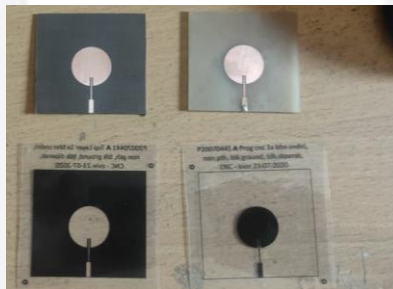
Gambar 3. 4 Realisasi Antena Patch Sirkular Tanpa Slot.
