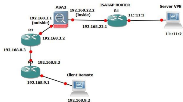
Gambar 3.2 Topologi jaringan remote access IPSec VPN
