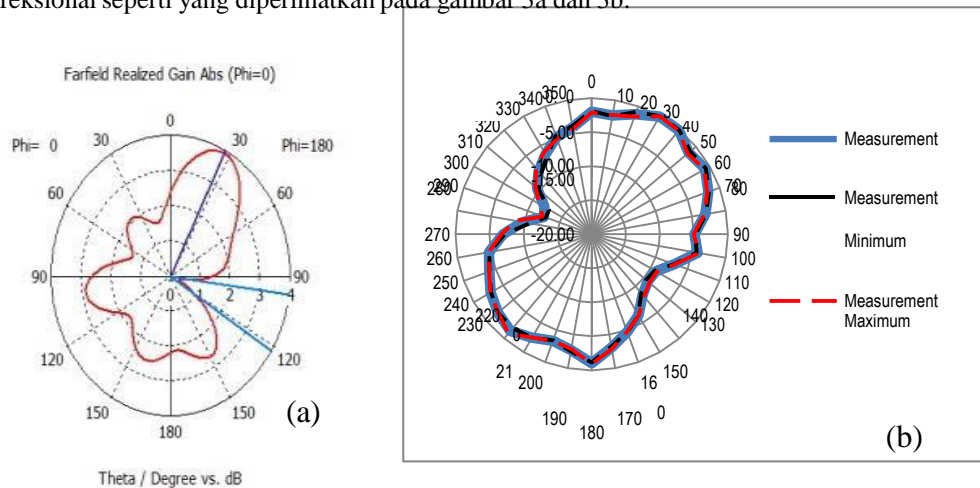
Gambar 3(a),(b): Pola Radiasi Azimuth Antena Cloverleaf
