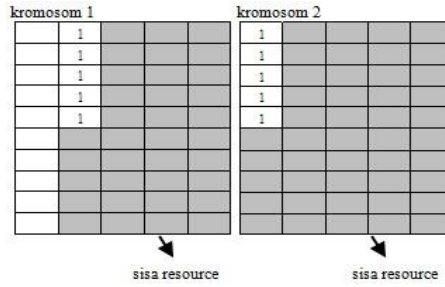
Gambar 8.Fungsi Nilai Fitness
