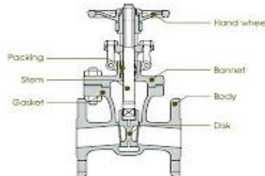
Gambar 1 Gate valve
