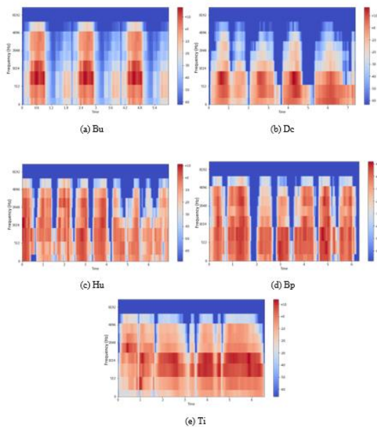
GAMBAR 7 Mel Spectrum
