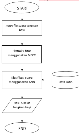
GAMBAR 5 Flowchart
