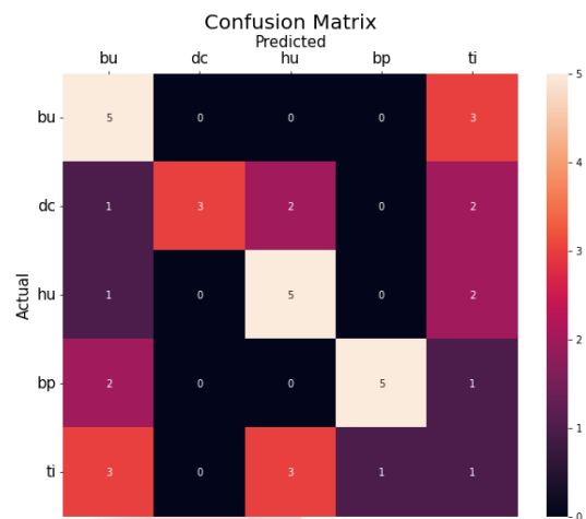
GAMBAR 9 Confusion Matrix
