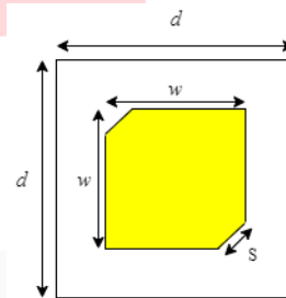
GAMBAR I DESAIN ANTENA SINGLE PATCH
