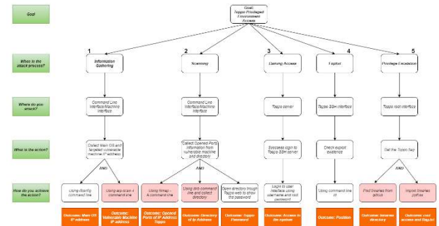
GAMBAR V.3 ATTACK TREE BERDASARKAN 5 WALKTHROUGH
