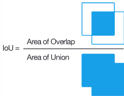
Gambar 9. Perhitungan IoU
