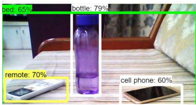
Gambar 1. Object Detection [6]
