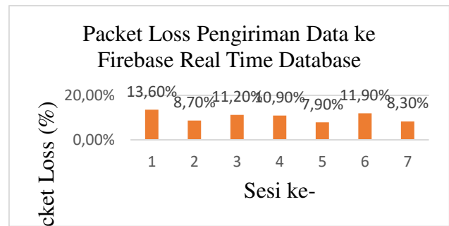
GAMBAR 14 Hasil Pengujian Packet Loss
